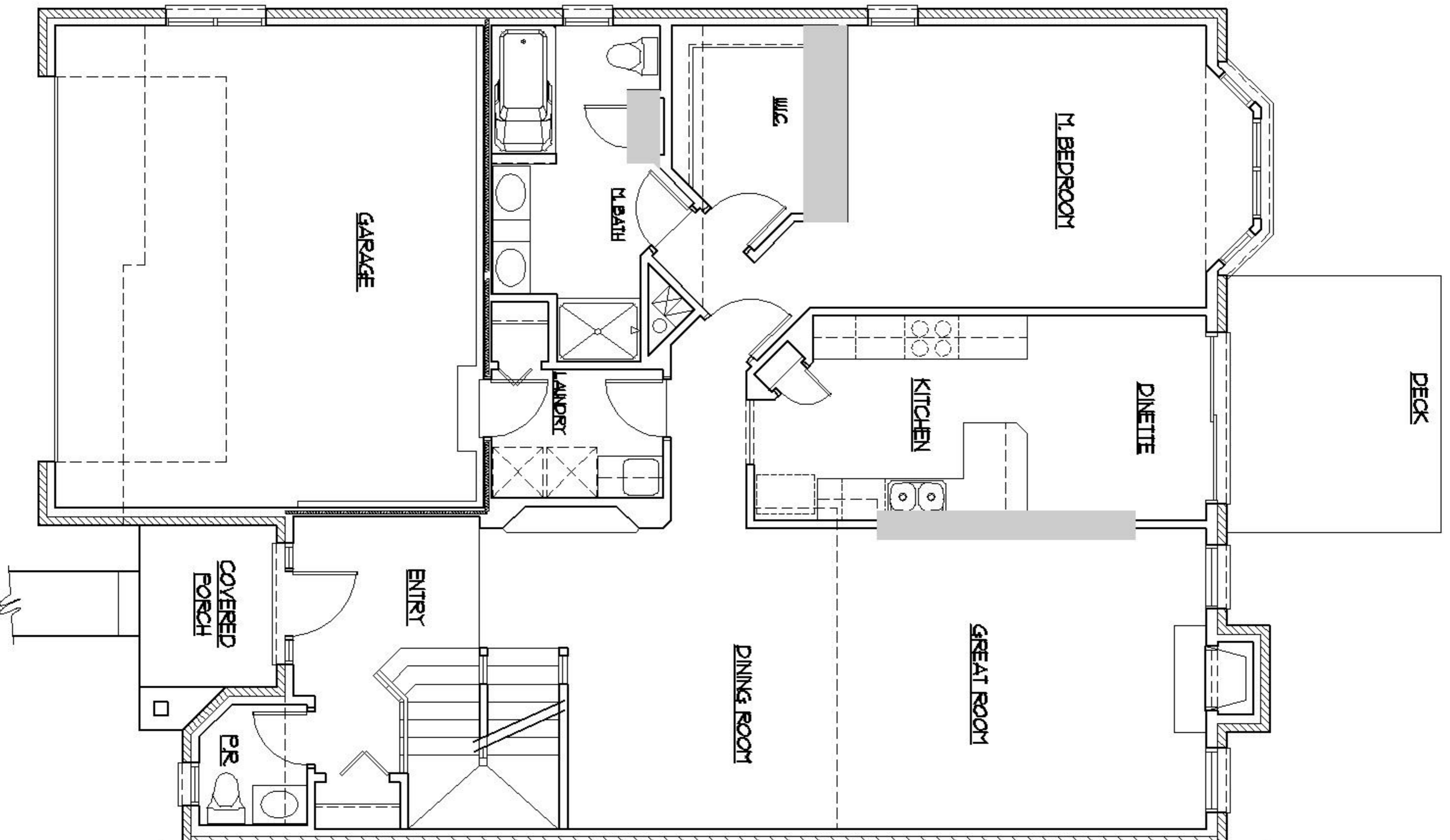
FIRST FLOOR PLAN SCALE: 1/4" = 1'-0" (LEFT END)
